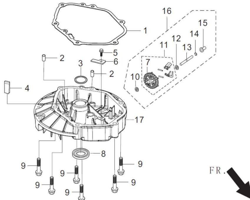
FIG.3 CRANKCASE COVER SUBASSEMBLY
